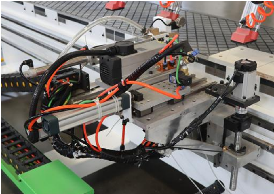
Drilling Spindle, Glue Injector & Dowel Insert Station
