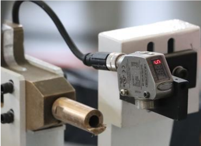
Dowel Insert & Photo Positioning Sensor
