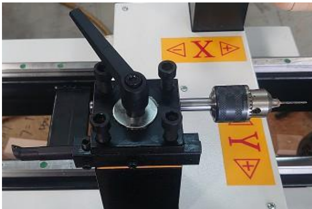
Tool Post # 1
