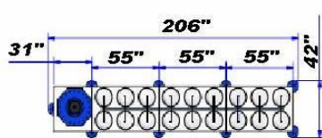
Standard Machine with 6 BIG top bags (Picture showing optional 18 Small top bags)
