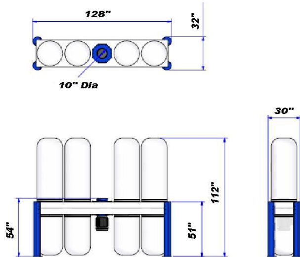
DC-9100 10HP 3PH Dust Collector
