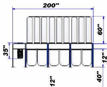
Standard Machine with 6 BIG top bags (Picture showing optional 18 Small top bags)
