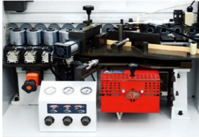
Hot Glue Tank Unit
