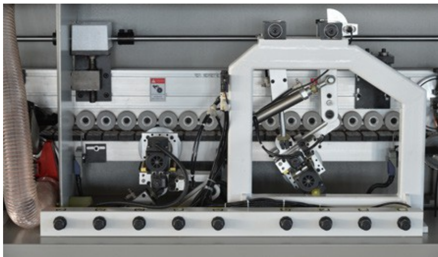
Conner Rounding /Tracing Station
